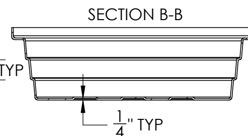
1 Drum Tray
